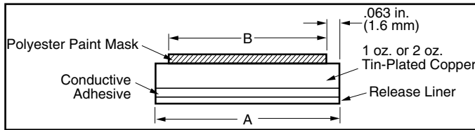
CHO-MASK® II - Construction
